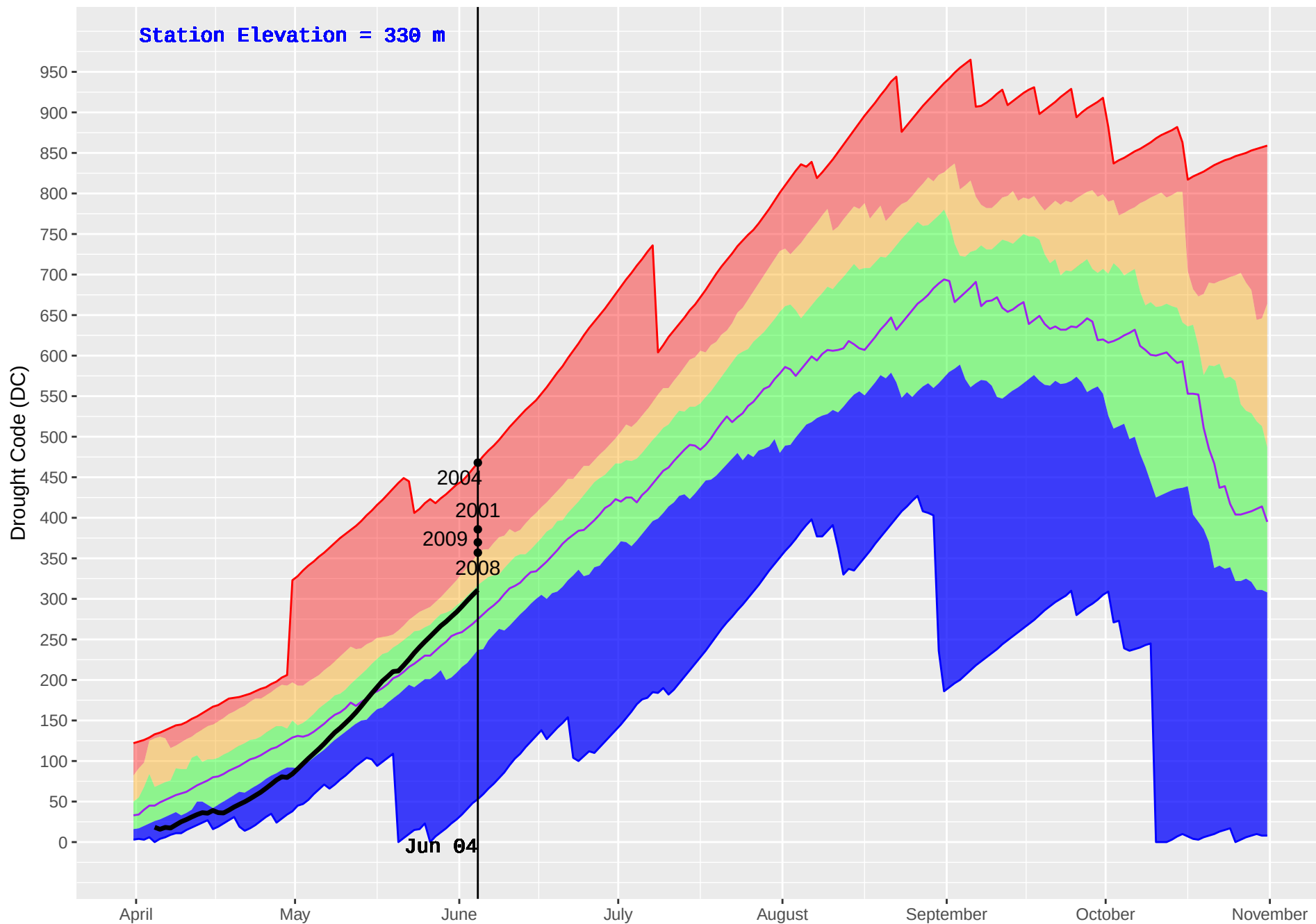
D'ARCY (292) : Historical (1978–2016) and Current (2018) Noon Drought Code (DC)
