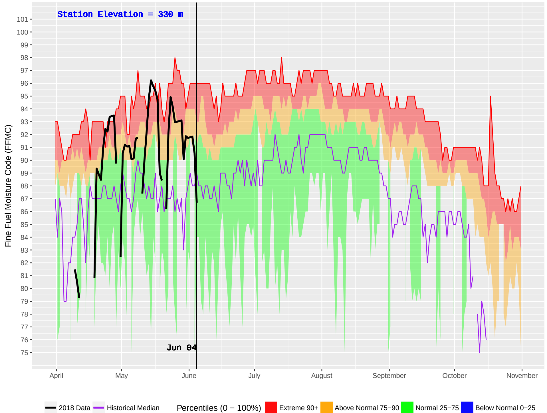
D'ARCY (292) : Historical (1978–2016) and Current (2018) Noon Fine Fuel Moisture Code (FFMC)
